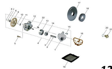
BOMBA ACEITE OIL PUMP
