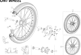
RUEDA DELANTERA FRONT WHEEL
