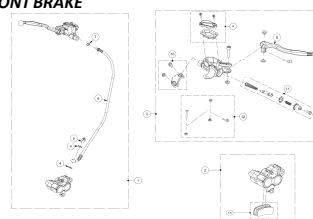
FRENO DELANTERO FRONT BRAKE
