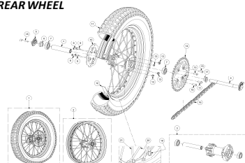
RUEDA TRASERA REAR WHEEL
