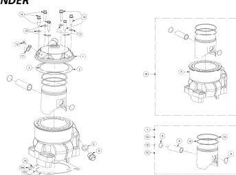
CILINDRO CYLINDER
