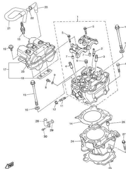
CILINDRO CYLINDER
