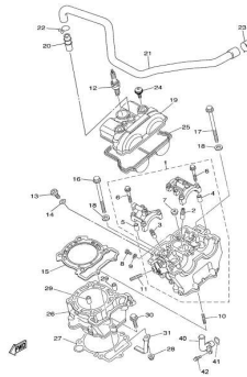
CILINDRO CYLINDER
