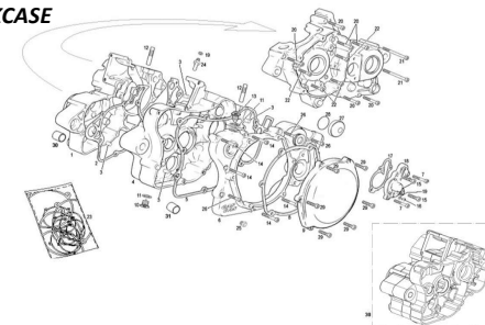
CARTER CRANKCASE
