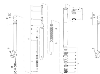
HORQUILLA DELANTERA FRONT FORK
