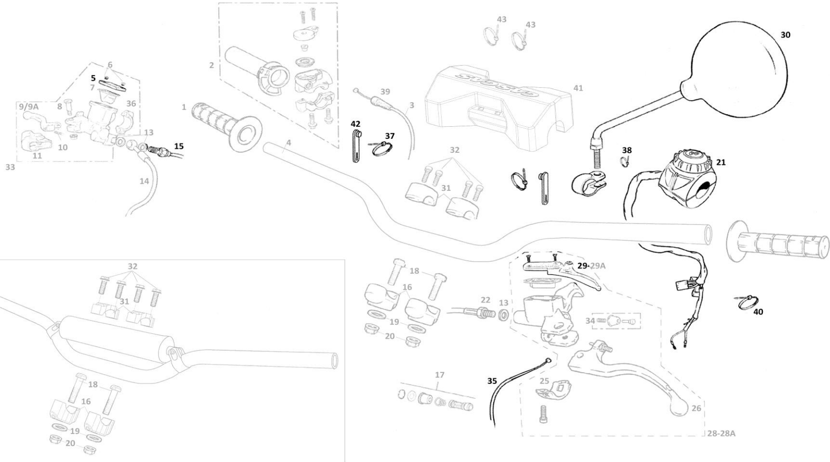
MANILLAR RACING / RACING HANDLEBAR
