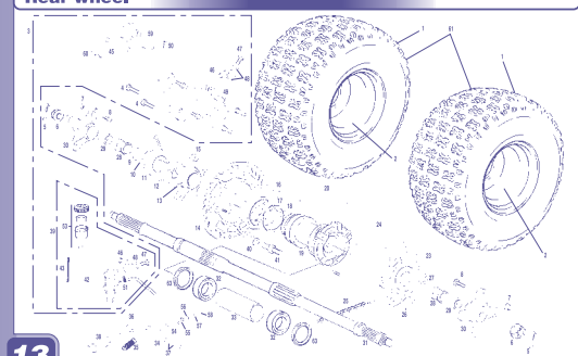
Rueda trasera / Rear wheel GASCAS WILD H.P.
