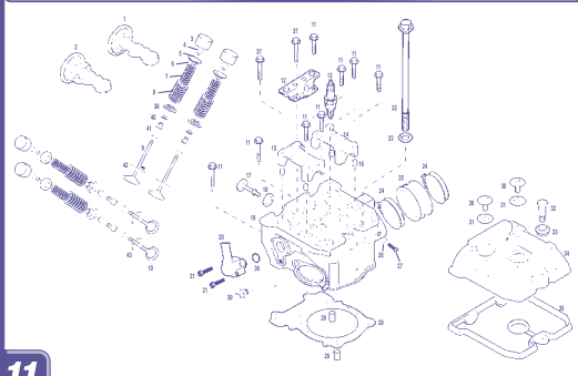
Culata / Cyl. head GAS GAS WILD H.P.
