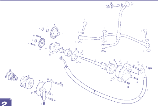
Bombas aceite / Oil pumps CASCAS WILD H.P.
