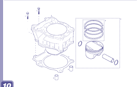
Cilindro / Cylinder GAS GAS WILD H.P.
