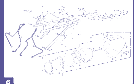
Filtro / Air filter GASGAS WILD H.P.
