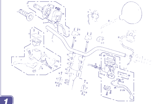
Manillar / Handlebar GASGAS WILD H.P.
