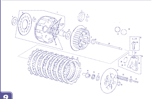
Embrague / Clutch GAS GAS WILD H.P.
