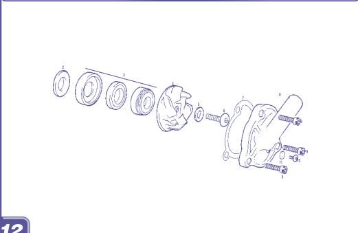
Bomba agua / Water pump GAS GAS WILD H.P.
