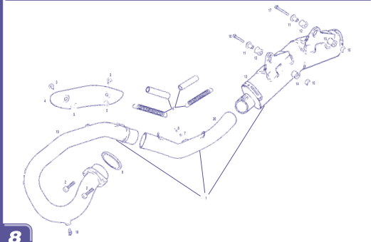
Tubo escape / Exhaust GASCAS WILD H.P.
