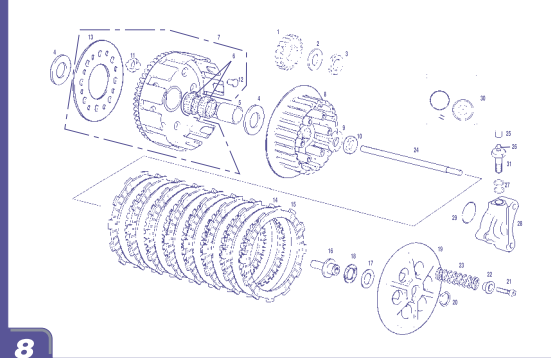
Embrague / Clutch GAS GAS WILD H.P.
