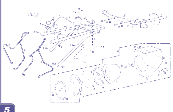
Filtro / Air filter CASCAS WILD H.P.
