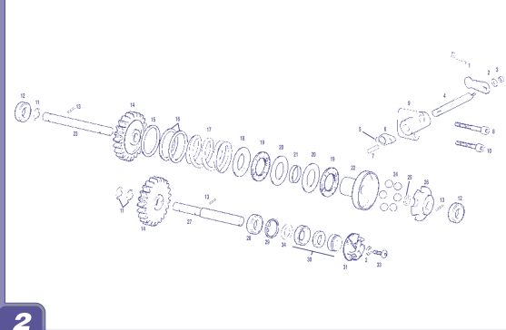
Centrifugo - Bomba / Impeller - Water pump GAS GAS WILD H.P.
