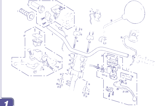
Manillar / Handlebar CASCAS WILD H.P.
