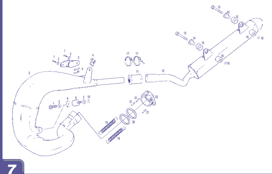
Tubo escape / Exhaust CASCAS WILD H.P.
