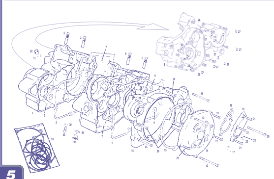
Cárter - Tapa embrague / Crankcase - Clutch cover GAS GAS WILD H.P.
