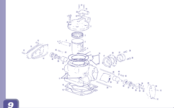
Cilindro - Culata - V. Escape / Cylinder - Cyl. head GAS GAS WILD H.P.
