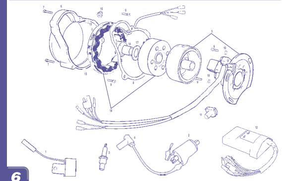
Encendido / Ignition GAS GAS WILD H.P.
