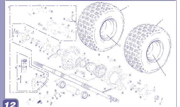
Rueda trasera / Rear wheel CASCAS WILD H.P.
