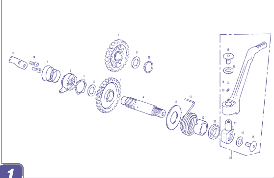
Conjunto pedal arranque / Kickstart set GAS GAS WILD H.P.
