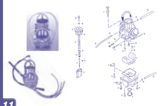
Carburador / Carburetor GAS GAS WILD H.P.
