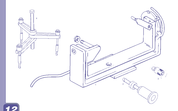
Utillaje / Tools GAS GAS WILD H.P.
