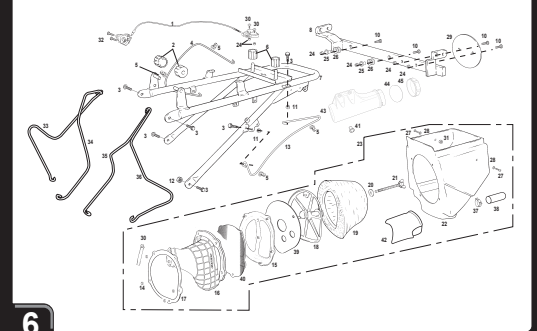
Filtro / Air filter CASGAS WILD HP
