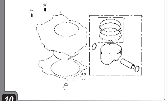
Cilindro / Cylinder GASGAS WILD HP
