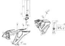
TANK
