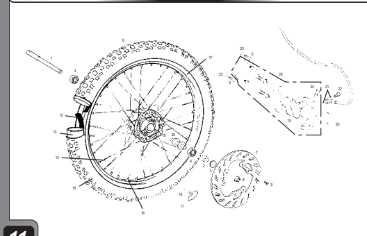
Rueda delantera / Front wheel GASGAS EC / SM ROOKIE 05
