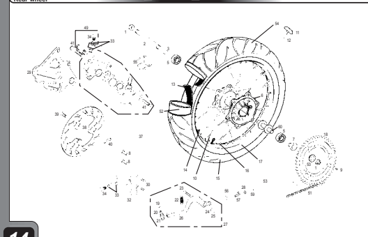
Rueda trasera / Rear wheel GASGAS EC / SM ROOKIE 05
