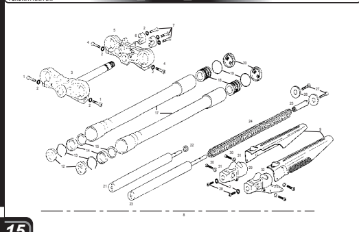
Suspension SHOWA / SHOWA Front Fork GASGAS EC / SM ROOKIE 05
