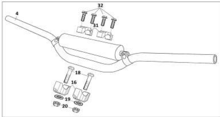
MANILLAR RACING / RACING HANDLEBAR
